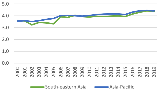
► Figure 8. CO2 emissions, 2000-2019, South-eastern Asia and Asia-Pacific (metric tonnes per capita)
