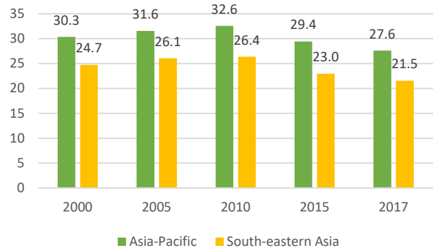
► Figure 9. Air quality PM 2.5 emissions, 2000-2017, South-eastern Asia and Asia-Pacific (micrograms per cubic metre)
