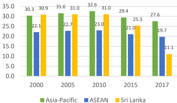
Figure 9. Air quality PM 2.5 emissions, 2000-2017, Sri Lanka, ASEAN and Asia-Pacific (micrograms per cubic metre)
