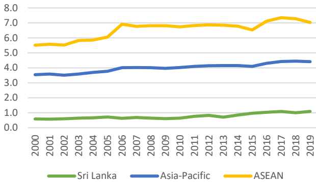
Figure 8. CO2 emissions, 2000-2019, Sri Lanka, ASEAN and Asia-Pacific (metric tonnes per capita)
