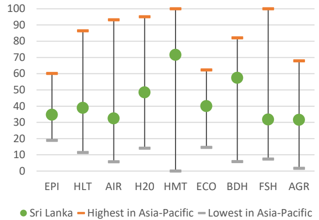
► Figure 5. Environmental performance index and selected indicators, Sri Lanka and Asia-Pacific, 2022
