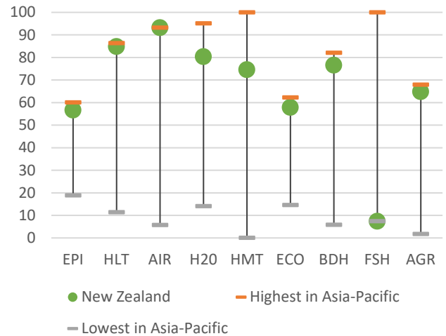
► Figure 5. Environmental performance index and selected indicators, New Zealand and Asia-Pacific, 2022
