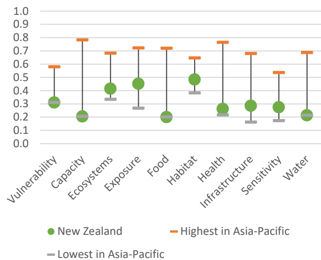
► Figure 10. Notre Dame Global Adaptation Index, Vulnerability and composite indicators, 2020, New Zealand, Asia-Pacific (index score)
