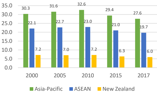
► Figure 9. Air quality PM 2.5 emissions, 2000-2017, New Zealand, ASEAN and Asia-Pacific (micrograms per cubic metre)
