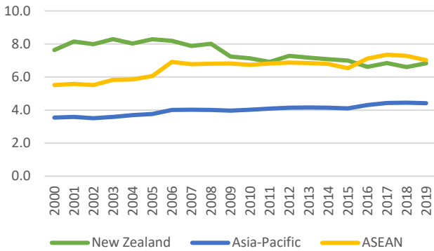
► Figure 8. CO2 emissions, 2000-2019, New Zealand, ASEAN and Asia-Pacific (metric tonnes per capita)
