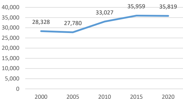
► Figure 12. Total renewable energy generation (GWh), 2000-2020
