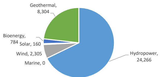
► Figure 13. Renewable energy generation (GWh) by technology, 2020
