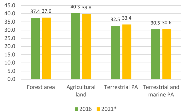
► Figure 7. Forest area, agricultural land, terrestrial and marine protection areas, 2016 and 2021 (percentage)
